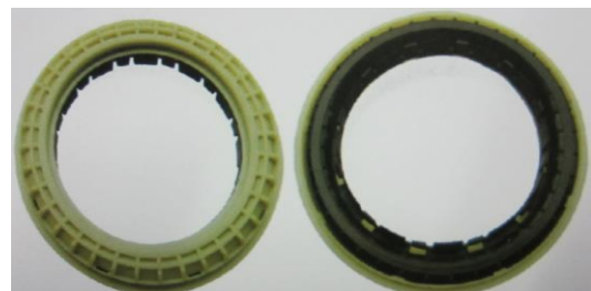
93220008 ID: 14mm OD: 119mm Thickness: 81.7mm
