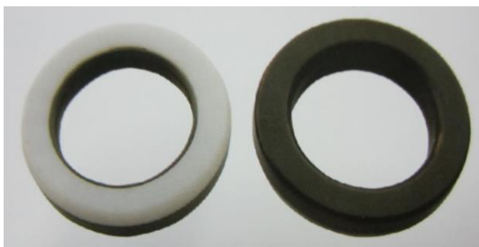
93220001 ID: 15mm OD: 78mm Thickness: 50.5mm
